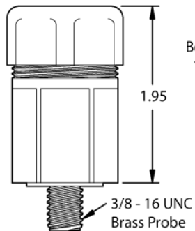
TT420S-LT 1/2" Straight
