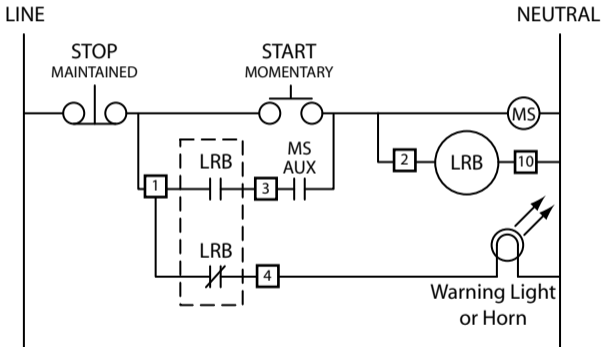
Figure 7: Typical Wiring Diagram
