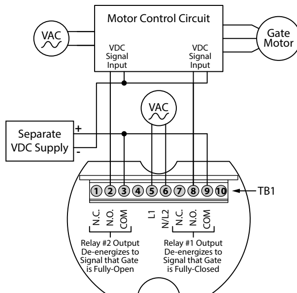
Figure 9: SG1000RA Relay Outputs with Vdc Wiring Configuration
