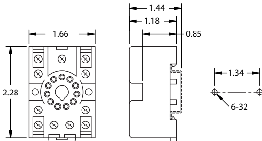
Terminal Block
